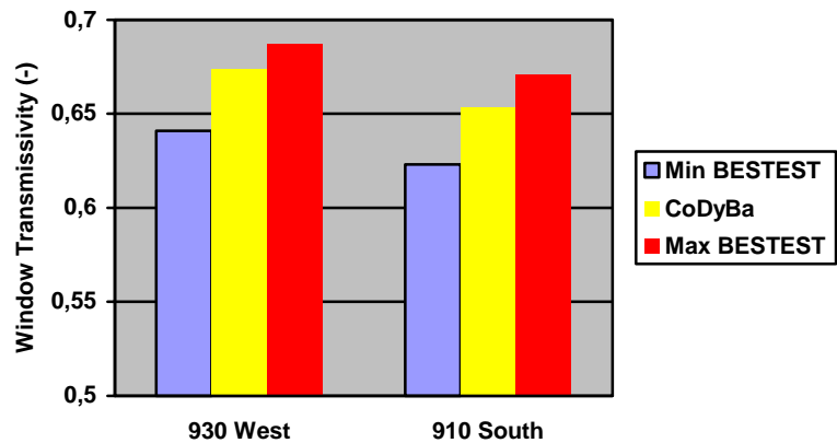
Fig. R4 : Annual Transmissivity Coefficient of Windows
